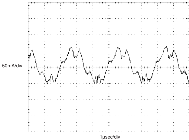
(VIN = 24V, 5V @ 15A, 3.3V @ 0A, external 22µF low-ESR input capacitor.)
