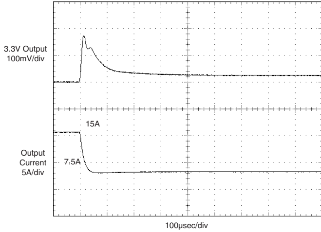
3.3V Output Full-Load to Half-Load Transient Response (VIN = 24V, 5V @ 0A, external 10µF || 1µF output capacitors.)
