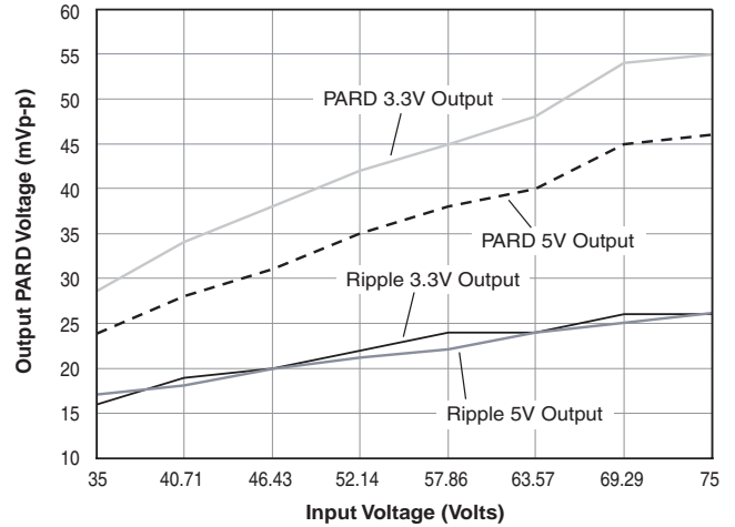
Output Ripple and Noise (PARD) vs. Input Voltage (One output @ 15A, other output @ 0A, PARD measured on loaded output, 20MHz bandwidth.)
