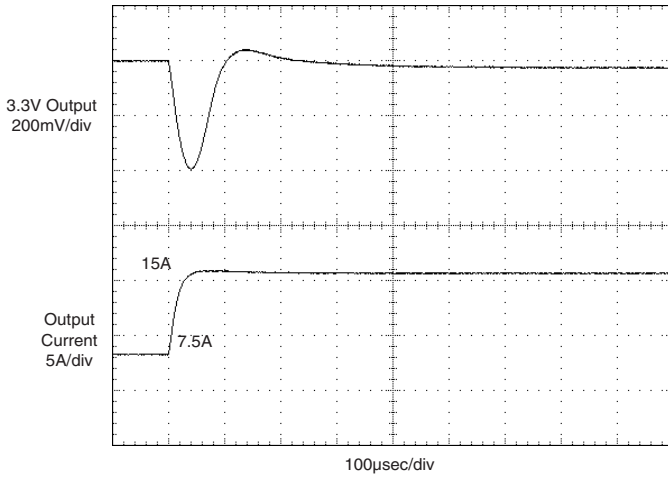
3.3V Output Half-Load to Full-Load Transient Response (VIN = 24V, 5V @ 0A, external 10µF || 1µF output capacitors.)
