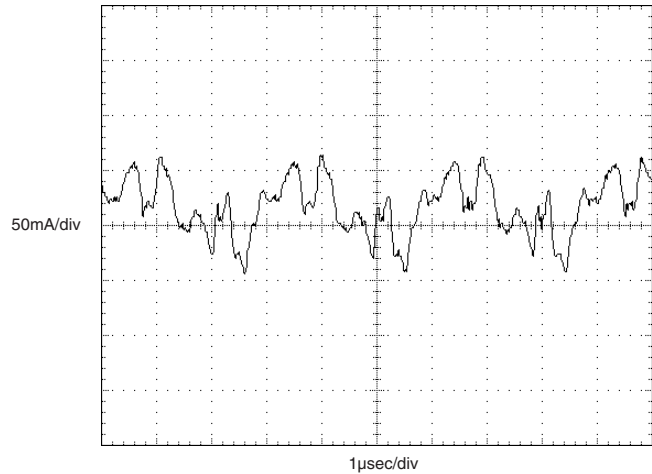
(VIN = 48V, 5V @ 15A, 3.3V @ 0A, external 22µF low-ESR input capacitor.)
