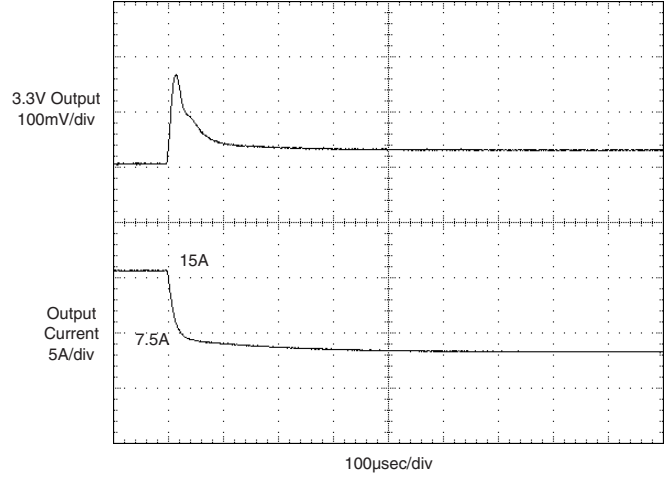
3.3V Output Full-Load to Half-Load Transient Response (VIN = 48V, 5V @ 0A, external 10µF || 1µF output capacitors.)
