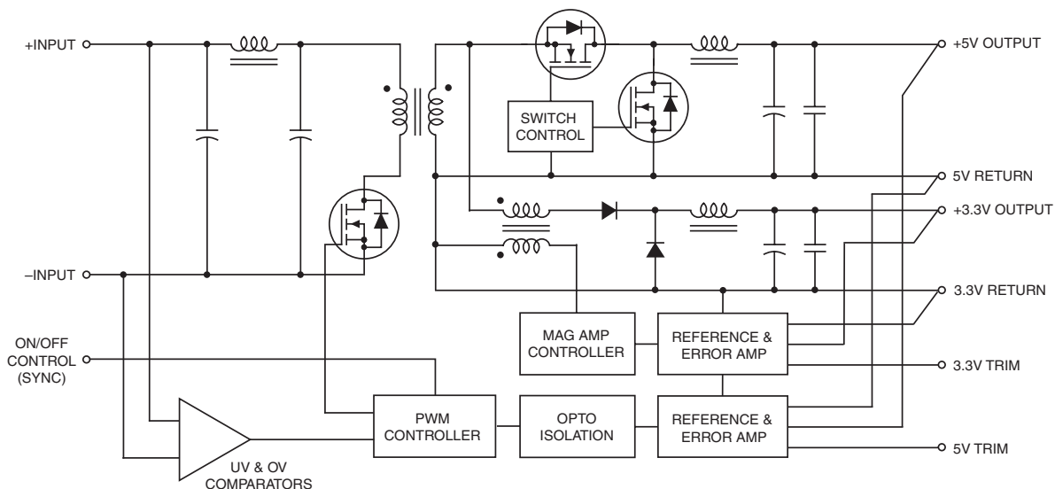
Figure 1. Simplified Schematic
